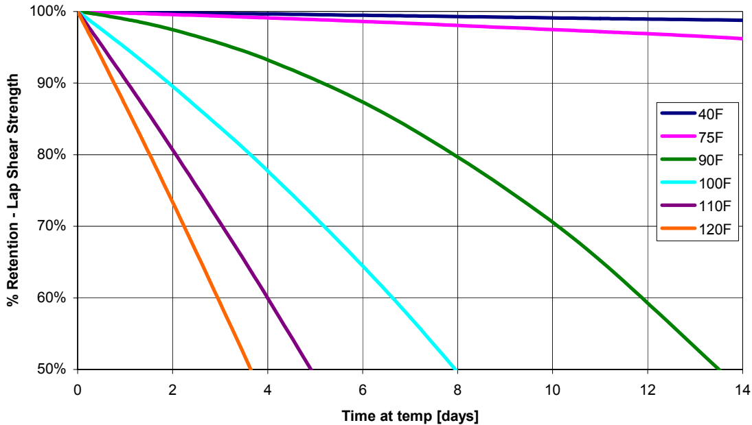
Figure 2 - Primerless Thermabond® stability at temperature (0 - 14 days)
