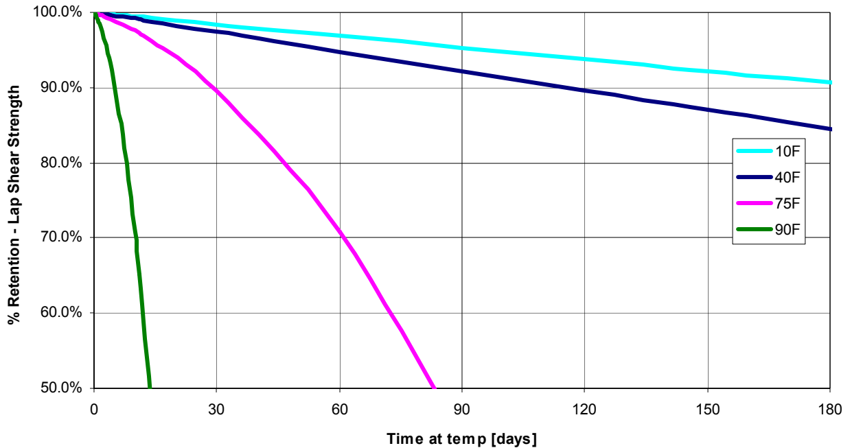
Figure 1 - Primerless Thermabond® stability at temperature (0 - 180 days)
